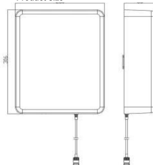
Product size
