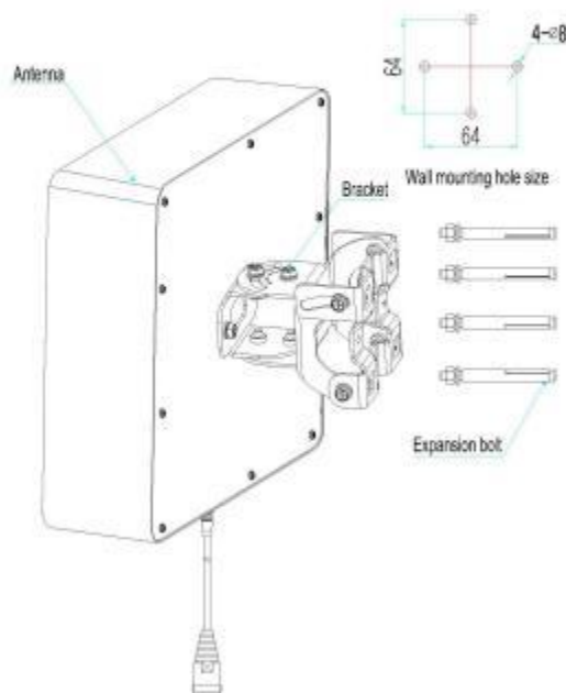
Wall Installation
