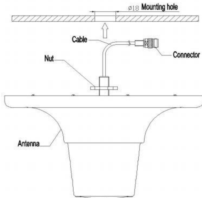
Installation Sketch
